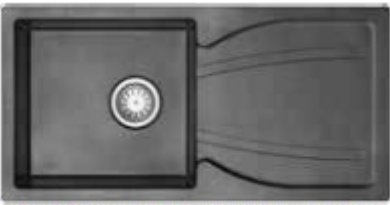
QI-007 • Single Bowl with Drainer Overall Size : 860x432x230mm (34"x17"x8") Bowl Size : 400x372mm Available Colors QMTS
